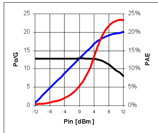
1900 MHz, 5V/70mA
