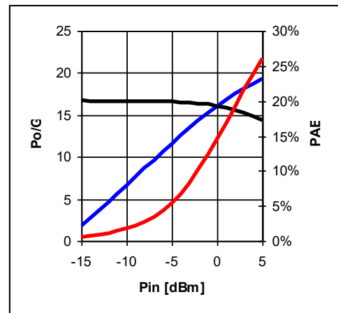
1900 MHz, 5V/55mA
