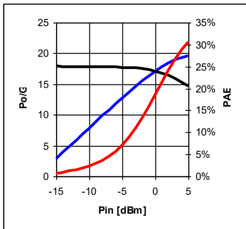
900MHz, 5V/55mA
